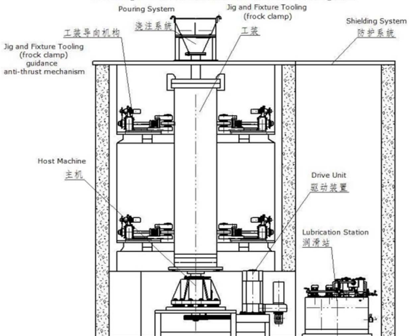
3556 Diagrammatic Sketch of Vertical CCM for Producing Rolls
