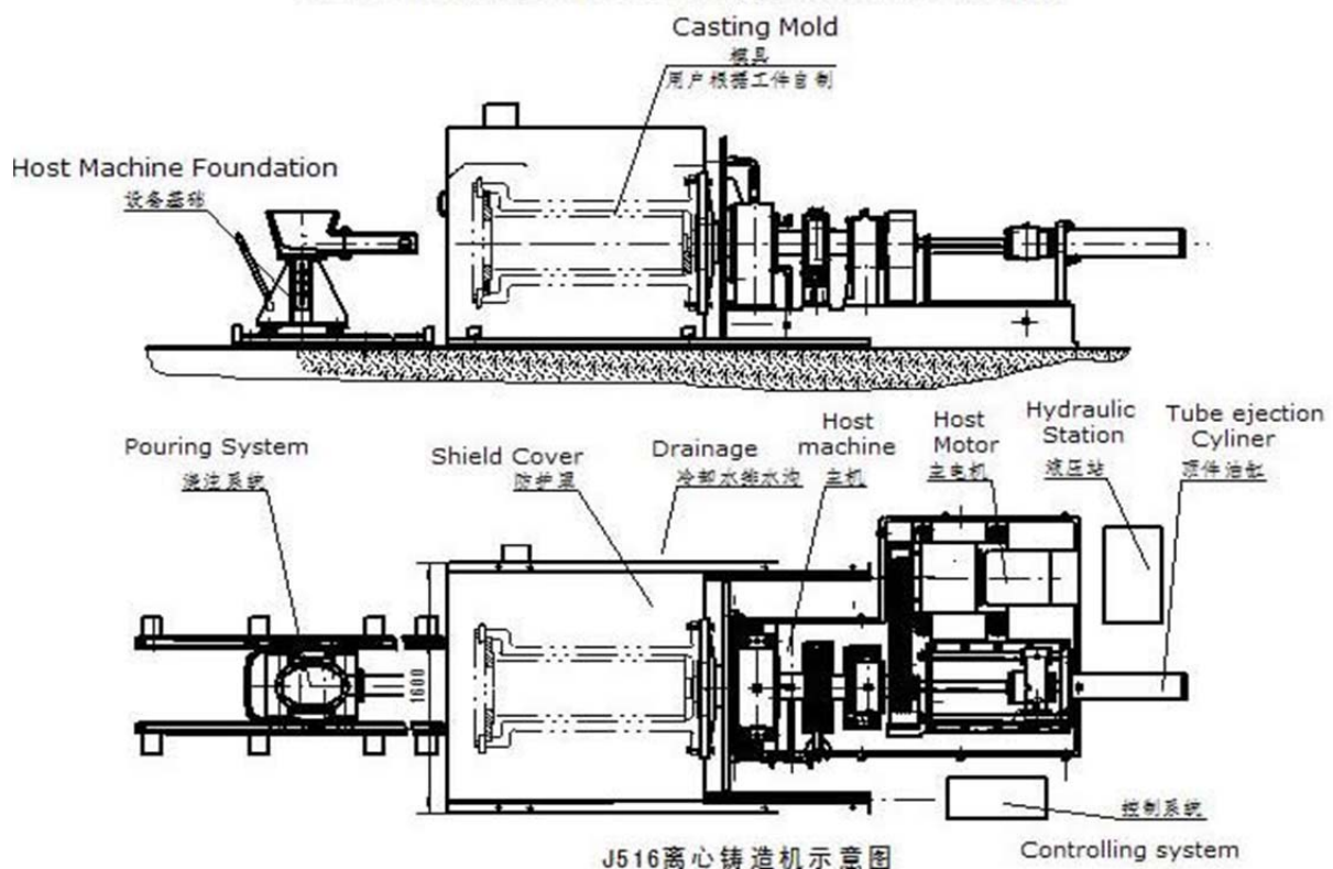
J516 Cantilever CCM Diagrammatic Sketch
